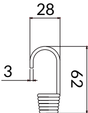
METALLIC GALVANIZED SPRING CATCH
