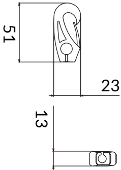
STANDARD SPRING CATCH
